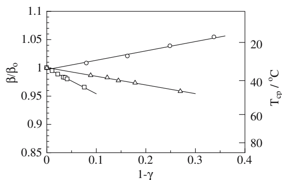
Fig. 3 T_{cp} and the reduced one \beta/\beta_0 as a function of 1-\gamma of PNIPAM for PNIPAM-AAm (squares), PNIPAM-HEMA (circles), and PNIPAM-DMAA (triangles) in water
