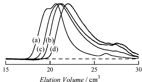
Fig. 1 GPC traces of PNIPAM (a), PNIPAM-AAm-4 (b), PNIPAM-AAm-5 (c), and PNIPAM-AAm-6 (d) in THF at 35^\circ\text{C}
