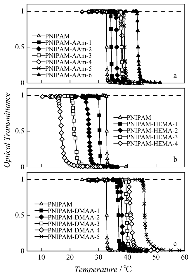
Fig. 2 Temperature dependence of OT of indicated copolymers in water ( c=5.00 \times 10^{-3} \text{ g cm}^{-3} ) for PNIPAM-AAm (a), PNIPAM-HEMA (b), and PNIPAM-DMAA (c)
