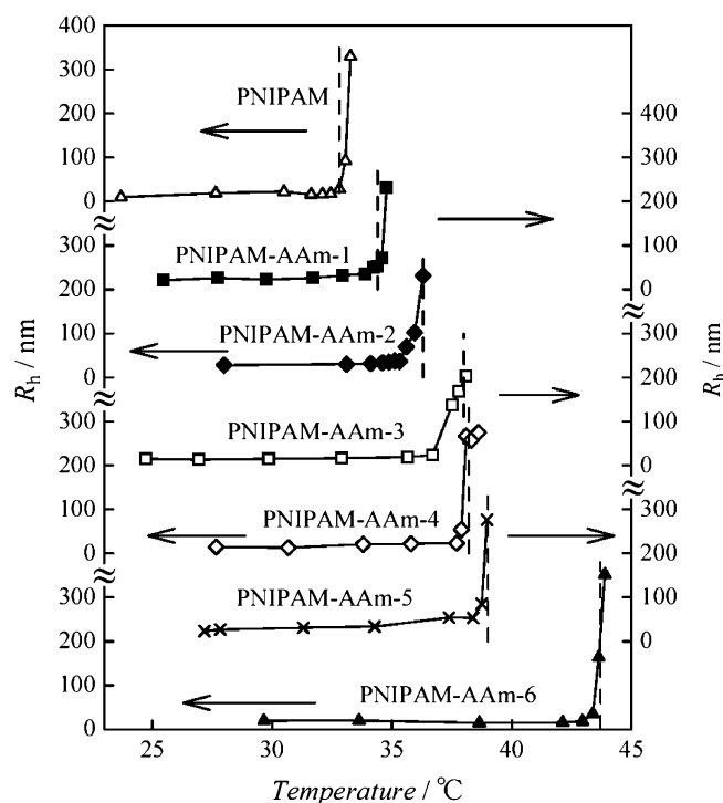
Fig. 4 Temperature dependence of R_h of indicated copolymers in water ( c=5.00 \times 10^{-3} \text{ g cm}^{-3} ). Dashed lines indicate T_{cp} for each sample
